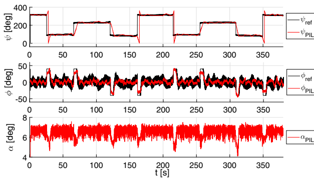
Fig. 20 PIL roll angle, heading angle and angle of attack
