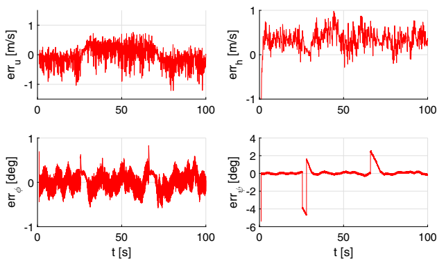
Fig. 22 PIL tracking errors for longitudinal velocity, altitude, and roll and heading angles
