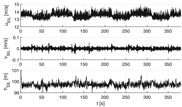
Fig. 11 SIL velocity components and altitude
