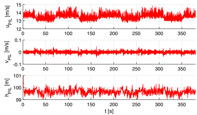
Fig. 18 PIL velocity components and altitude
