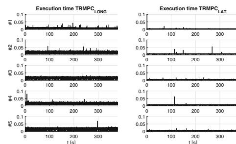
Fig. 25 SIL execution time [s]
