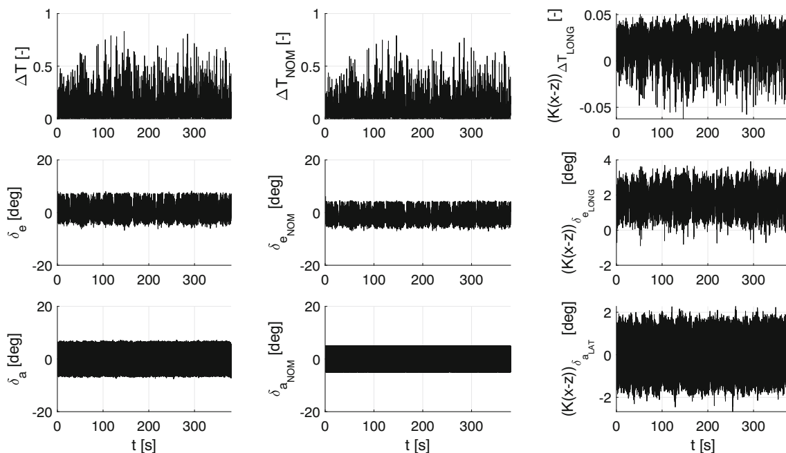
Fig. 16 SIL throttle and elevator and aileron deflections: (i) real (1st column); (ii) nominal (2nd column); and (iii) error component (3rd column)
