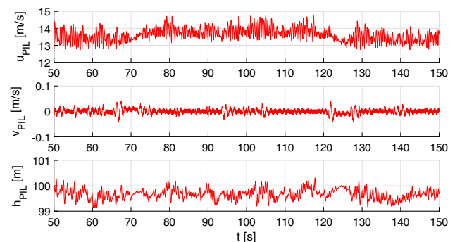
Fig. 19 Zoom-in on PIL velocity components and altitude
