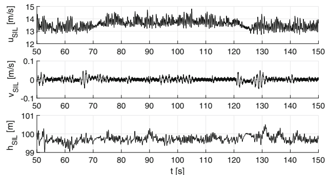
Fig. 12 Zoom-in on SIL velocity components and altitude
