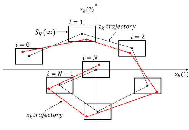
Fig. 6 Outer-bounding tube representation at the k -th time step over a prediction horizon of N
