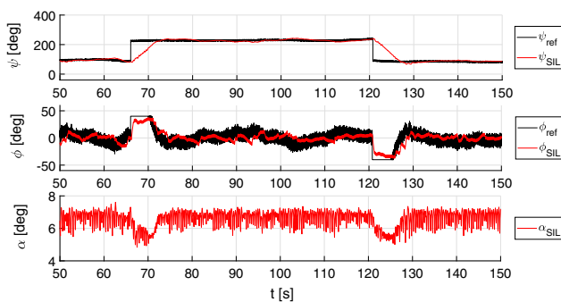
Fig. 14 Zoom-in on SIL roll angle, heading angle and angle of attack
